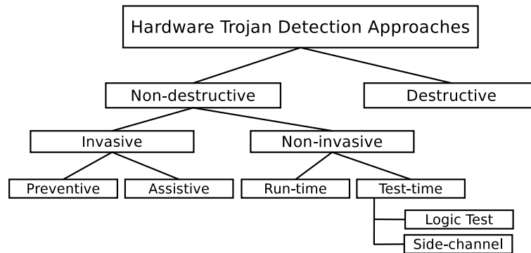
Figure 5: Hardware Trojan Detection Techniques: Chakraborty, Narasimhan & Bhunia (2010)
